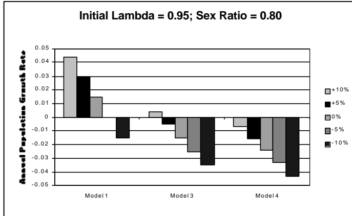
Figure 24. Annual population growth rates increases and decreases in the annual pelagic juvenile survival rate (-10%, -5%, 0%, +5% and +10%) and a 30% decrease in mortality for small benthic juveniles only (no expanded TED regulations). Models were based on pre-1990 population growth rates of -5%, -3% and 0% (equivalent to \lambda values of 0.95, 0.97 and 1.0). Proportion of female offspring is 0.80.
